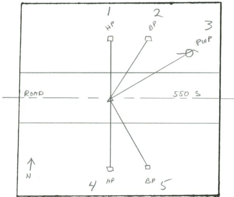
GRAPHIC TIES (SKETCHED)
